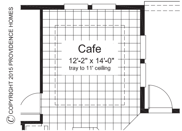
9. TRAY CEILING AT CAFE
